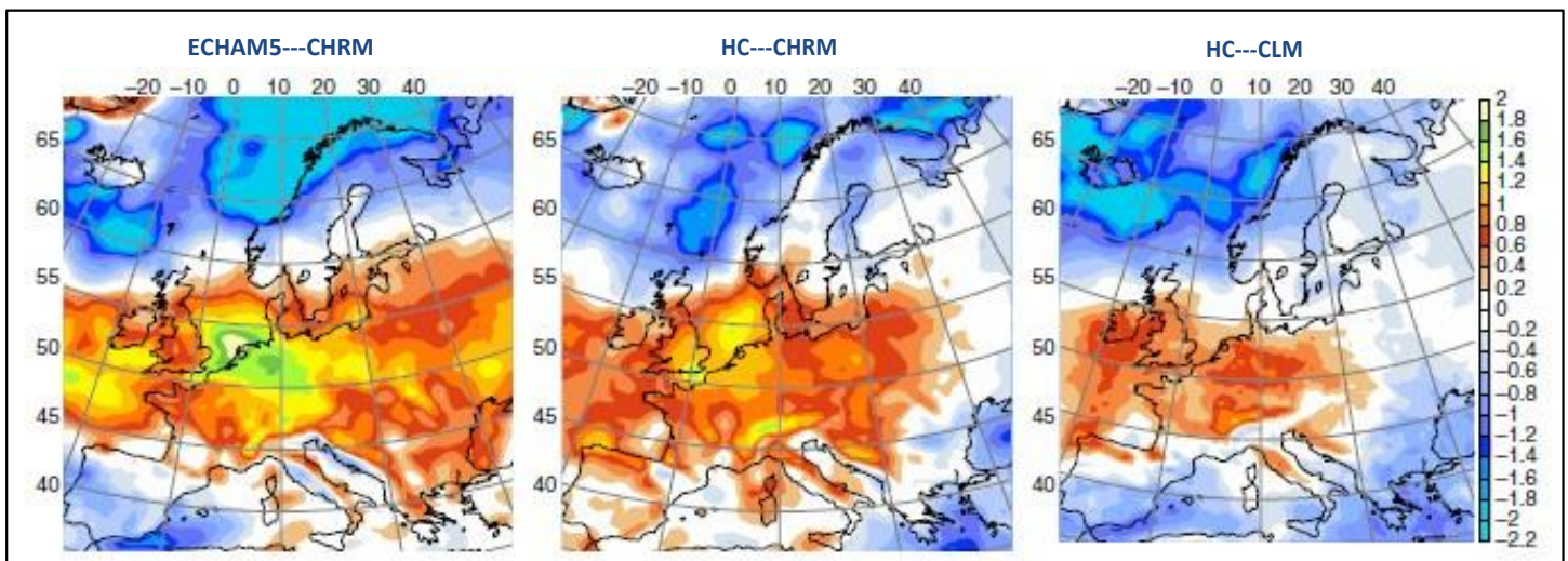
Figure 10. Expected climate change impact on ETC gust fields. Shown is the difference between historical CTL scenario (Oct 1961-Mar 1990) and the futuristic A2 scenario (Oct 2071-Mar 2100) set forth by the IPCC. Each box represents a different comparison of mean gust fields, given the three global climate model simulations (from left to right, ECHAM5-CHRM, HC-CHRM, HC-CLM).
