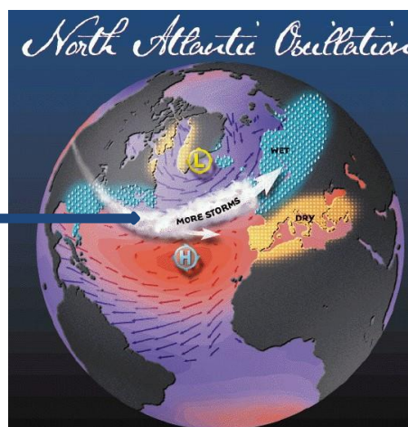
Figure 4. Positive phase of North Atlantic Oscillation.
