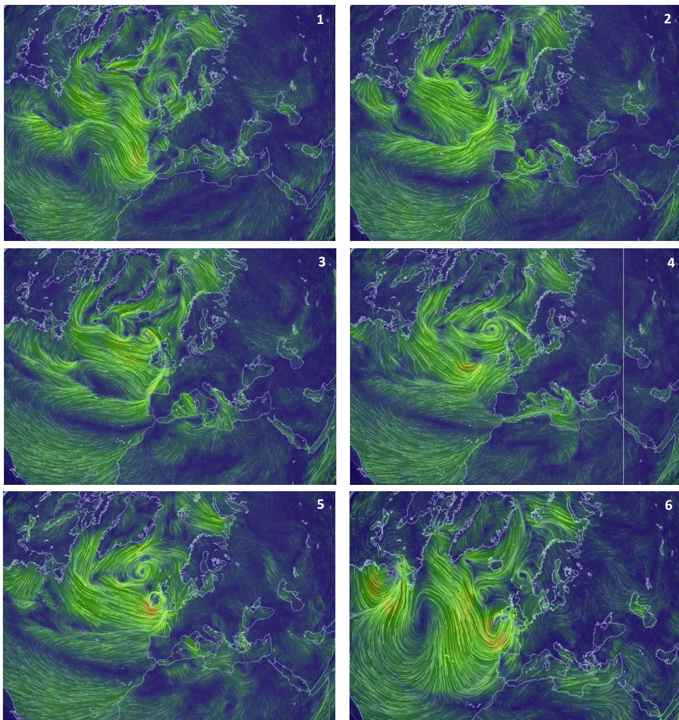
Figure 1. An extratropical disturbance turns into an organized storm in the eastern North Atlantic. Over February 12-14, 2014, a series of storms struck the coastline of northern Europe, causing widespread flood and damage, resulting in approximate insured losses of $1.3B to residences, businesses and infrastructure.
