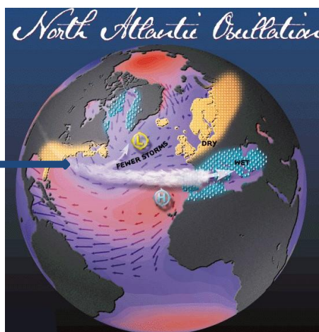
Figure 5. Negative phase of North Atlantic Oscillation.
