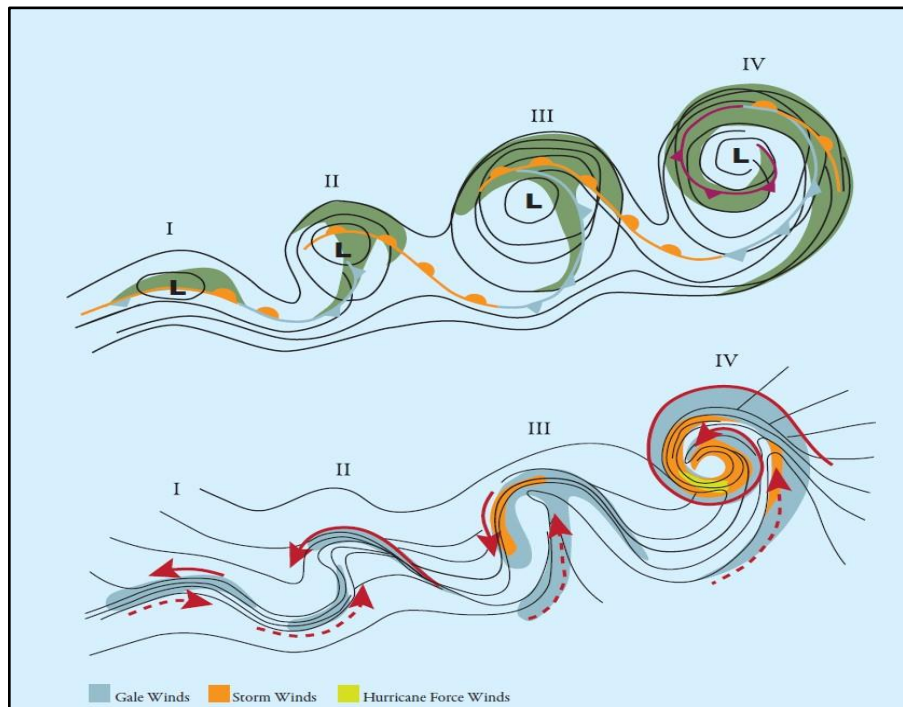
Figure 6. The Shapiro-Keyser Extratropical Cyclone Model, developed in 1990 shows the life-cycle of an ETC.
