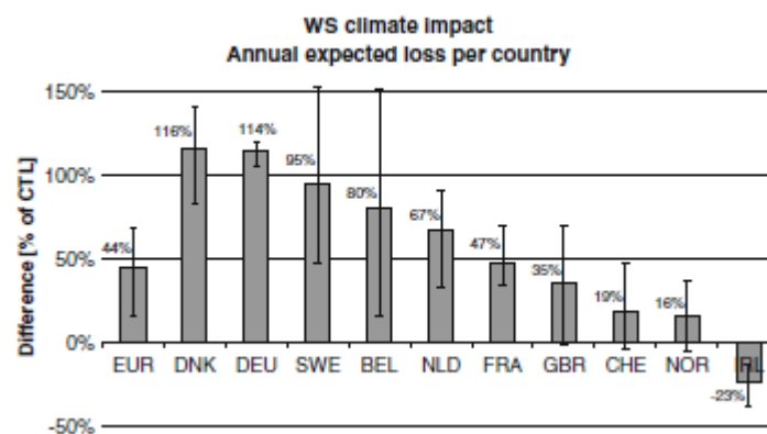
Figure 11. Climate change impact on annual expected loss, for selected regional markets given Swiss Re's insurance loss model. Error bars encompass results of the three model chains considered. (CTL=Control).
