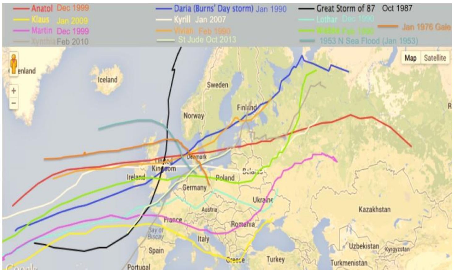
Figure 8. The various storm tracks of those listed in Table 1. The normal path of most storms is from the west-southwest to the east-northeast. The remaining storms without the aforementioned path take unusual routes through the North Atlantic and Europe.
