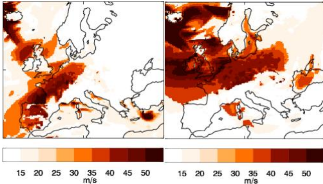
Figure 7. This shows the windstorm footprints of Xynthia (Feb 2010) on the left and Kyrill (Jan 2007) on the right. Although each storm had a slightly different storm track, one can see how the storms did not lose energy over land and were able to maintain strength deep into the European continent. Xynthia traveled over 1700 miles into Europe, Kyrill covered over 1800 miles.
