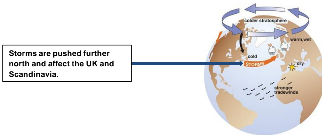
Figure 2. Positive phase of Arctic Oscillation.
