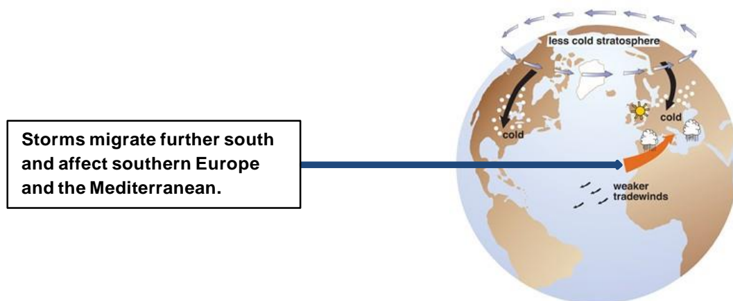
Figure 3. Negative phase of Arctic Oscillation.
